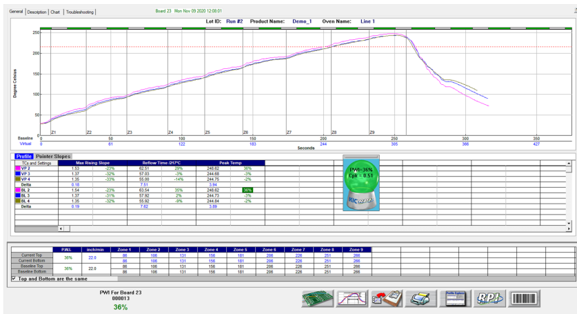
Temperature Graph and Data for Each PCB Processed
